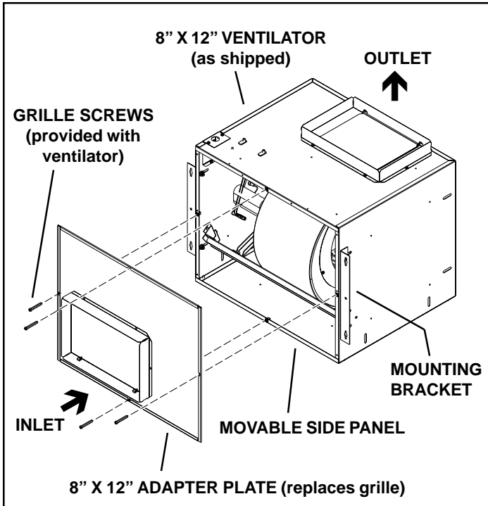
8" X 12" VENTILATOR Right Angle Discharge
