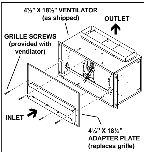
4½" X 18½" VENTILATOR Right Angle Discharge
