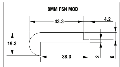
Stair Nose Dimensions
