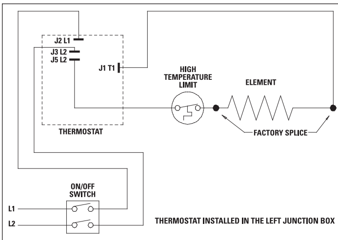
FIGURE "A" (Left Junction Box Wiring)
