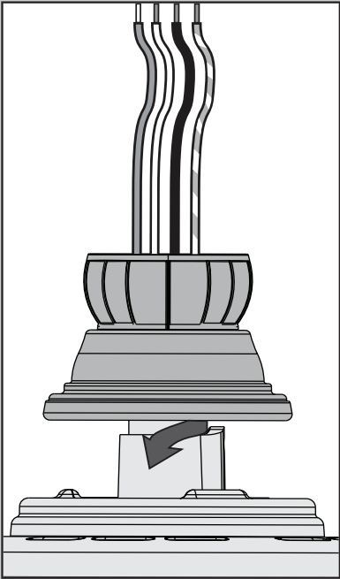
Slide the adapter cover onto the downrod, then hand tighten the downrod (at least 4-5 full turns) until it stops.
