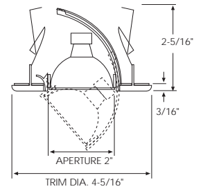
Adjustable Elbow Wallwash Downlight Trim
