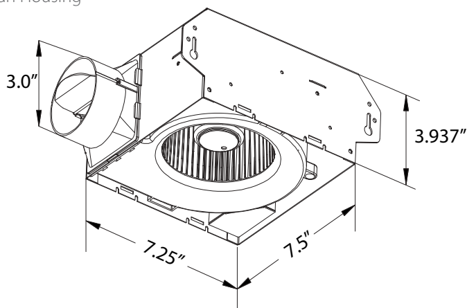
Fan Housing
