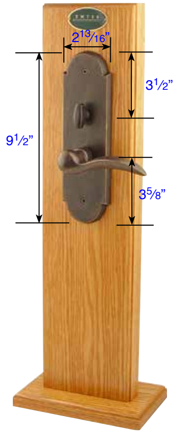
Standard interior trim Part # 3323*
