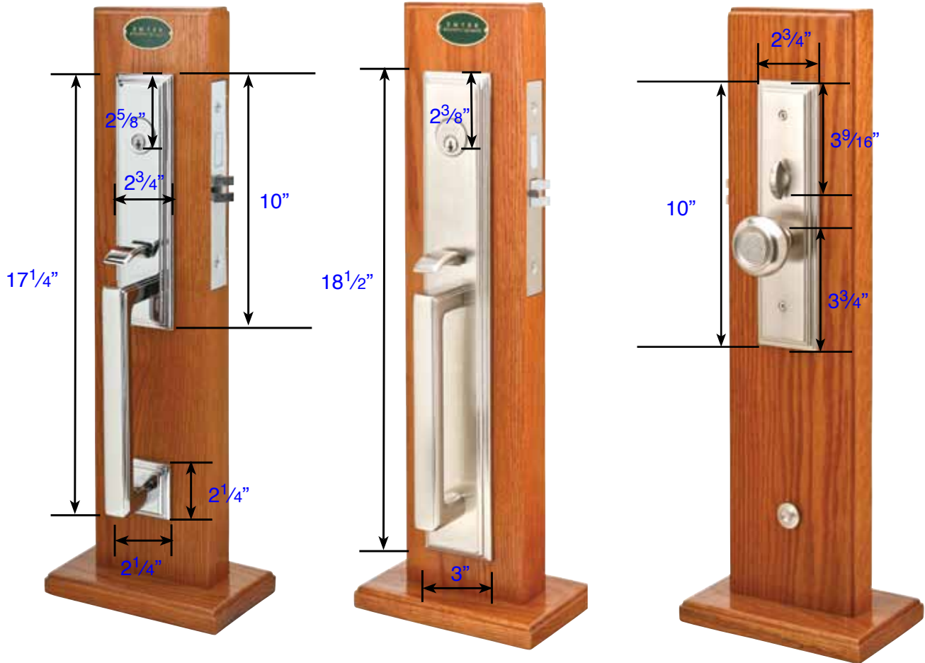
Manhattan Trim Style Part # UL 3306
