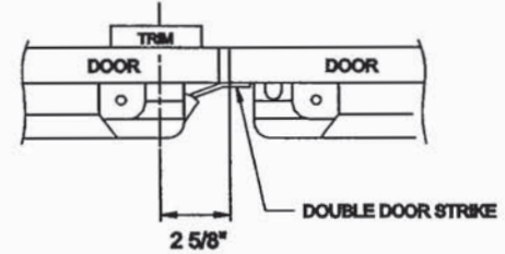
C. DOUBLE DOOR WITHOUT MULLION
