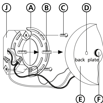
Drawing 2 - Final Assembly
