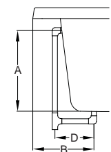
Drain/Overflow
