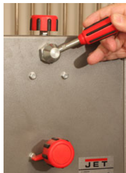
The blade wheels (left) are balanced and mounted on ball bearings for smooth running. We included easy blade tensioning (right) as well as a single lever for relaxing blade tension when not in use.
