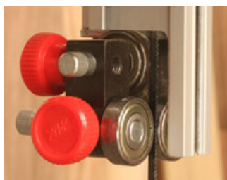
The upper and lower blade guides use ball bearings with tool-free adjustments!
