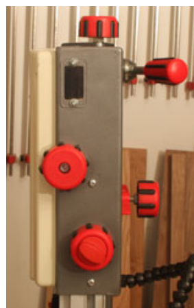
The controls are grouped for easy use. Note the blade tracking window that makes that adjustment easier and more accurate.
