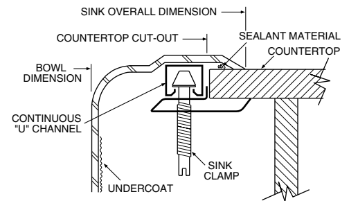
Installation Detail
