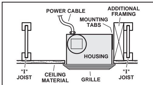
HOUSING MOUNTED TO "1" JOIST Requires additional framing for mounting tabs.
