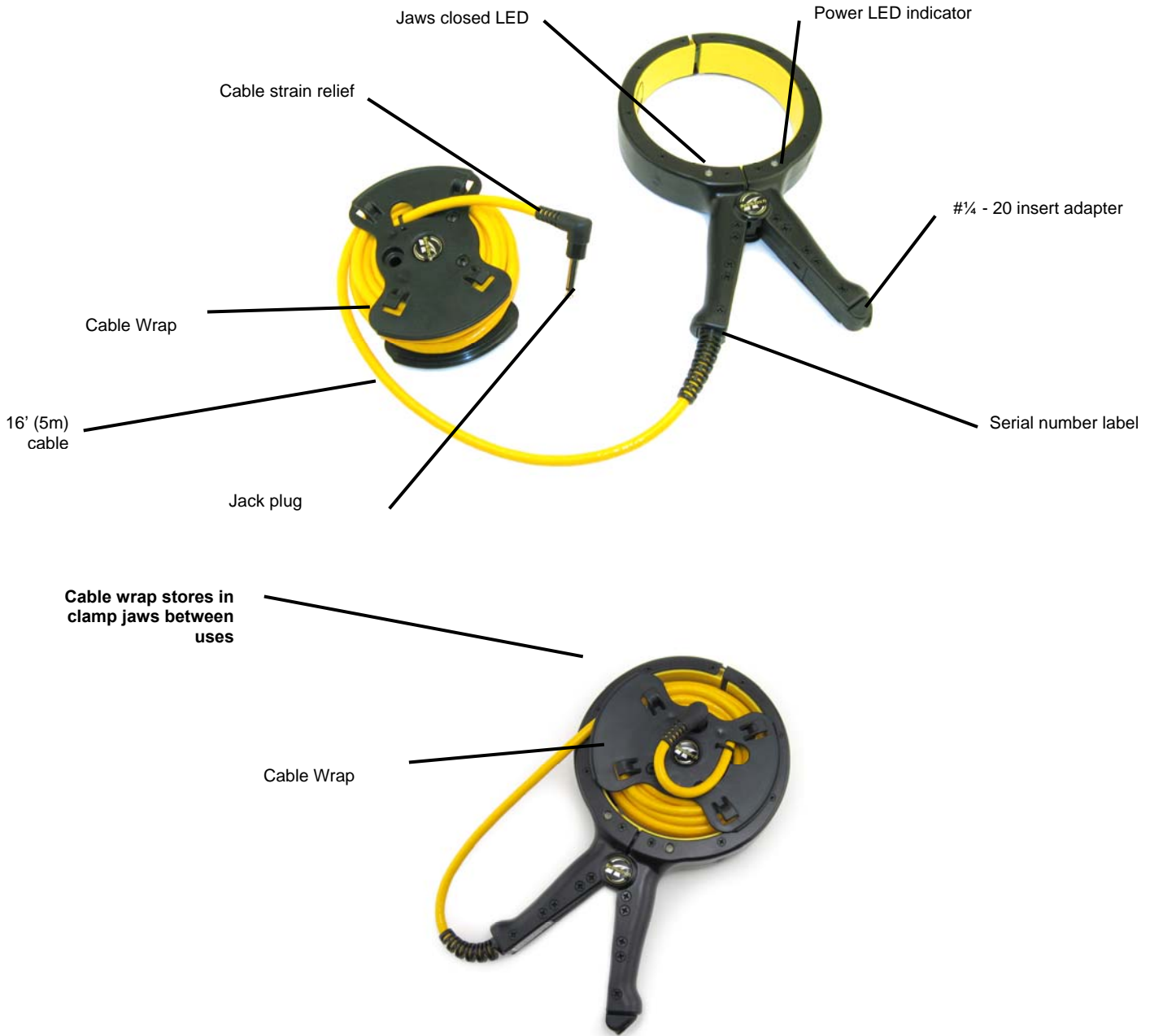
Figure 2: Inductive Clamp Components
