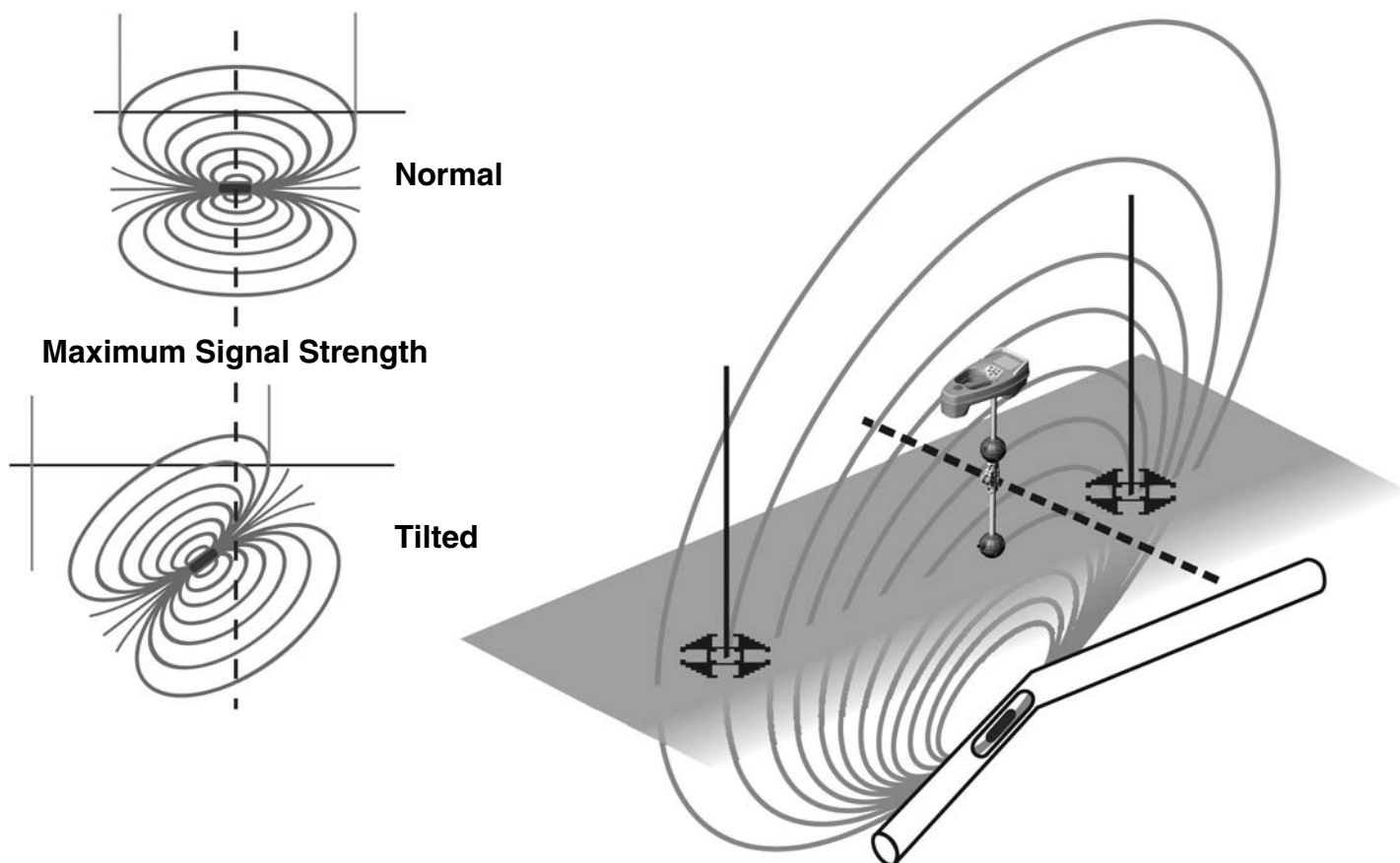
Figure 25 – Tilted Sonde, Poles and Equator
