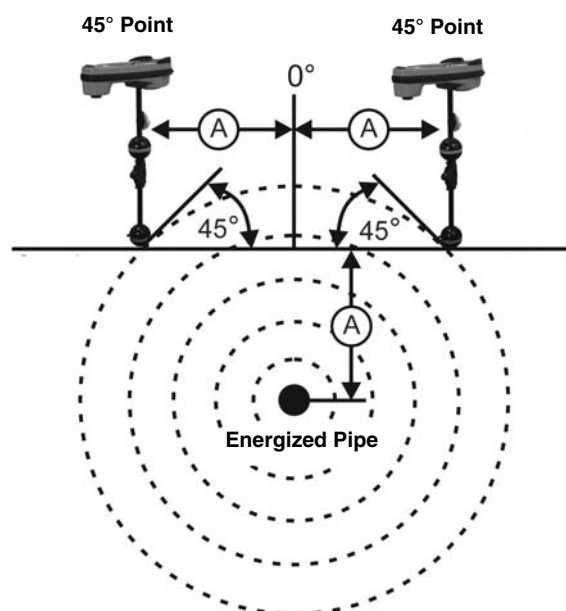
Figure 30 – Checking for Distortion
