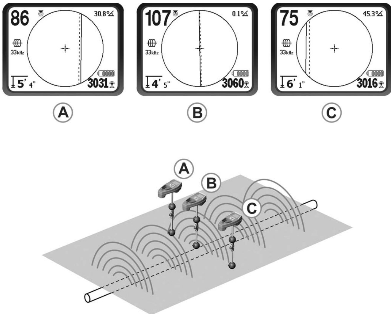
Figure 28 – Screen Display in Different Locations (Active Line Tracing)
