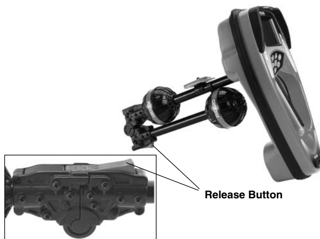
Figure 5 – Folding Antenna Mast and Release Button
