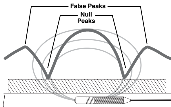
Figure 49 – The signal from a Sonde as “seen” by a conventional locator
