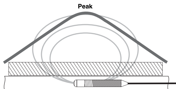
Figure 50 – Sonde signal as “seen” by the NaviTrack II
