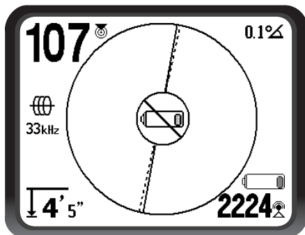
Figure 10 – Display Low-Battery Warning
