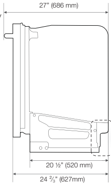
Side view (DMT800 series/ DMT610 series/ DMT400 series)
