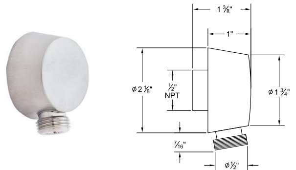
7089SE __ Supply Elbow
