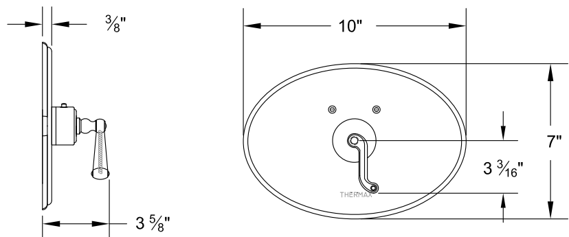
7093AN__ -TM Thermax Thermostatic Control Trim
