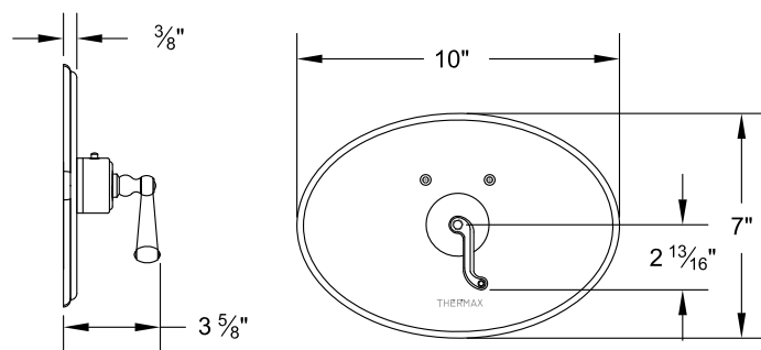
7093CA__TM Thermax Thermostatic Control Trim
