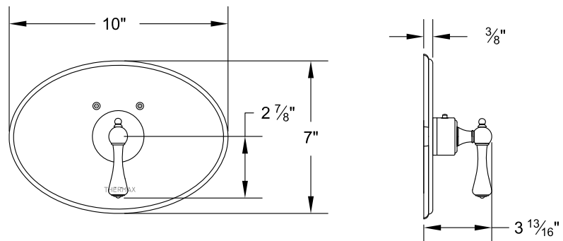
7093DD__-TM Thermax Thermostatic Control Trim
