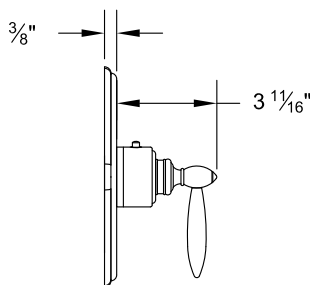
7093LA__ -TM Thermax Thermostatic Control Trim
