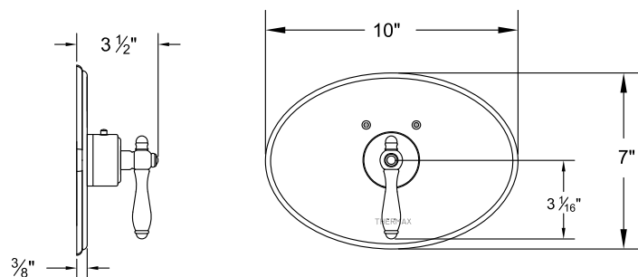
7093JZ_-TM Thermax Thermostatic Control Trim
