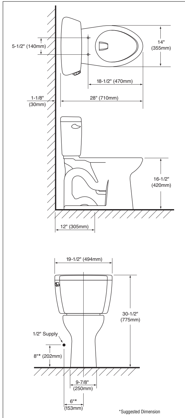
CST744EL - Eco Drake® Toilet, ADA Model
