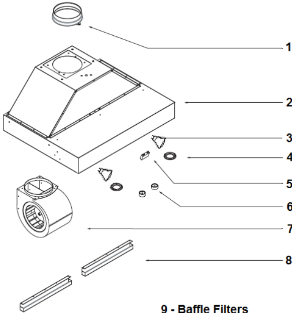
9 - Baffle Filters
