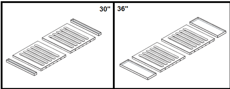
9 - Baffle Filters
