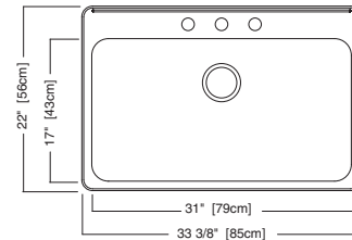
17SB.332283.073 Standard drilling: 3 hole
