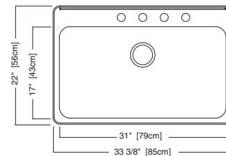
17SB.332284.073 Optional drilling: 4th hole on right
