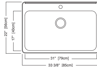
17SB.332211.073 Optional drilling: 1 hole on center
