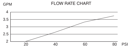
FLOW RATE CHART
