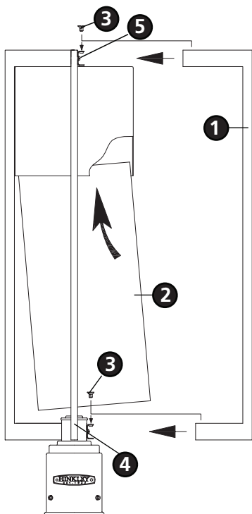
Drawing 2 - Glass Replacement
