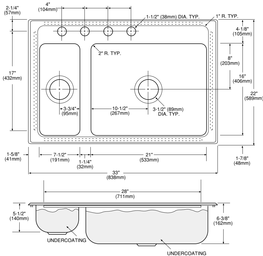
Installation Detail
