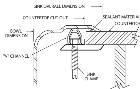
Installation Detail
