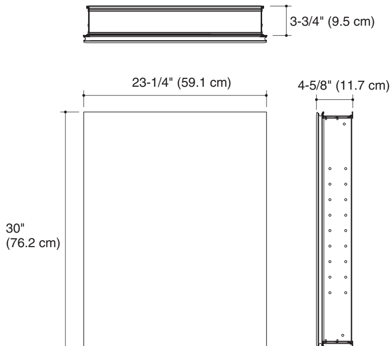
Product Diagram
