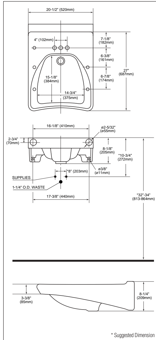
LT308.4 - Wheelchair Users Lavatory
