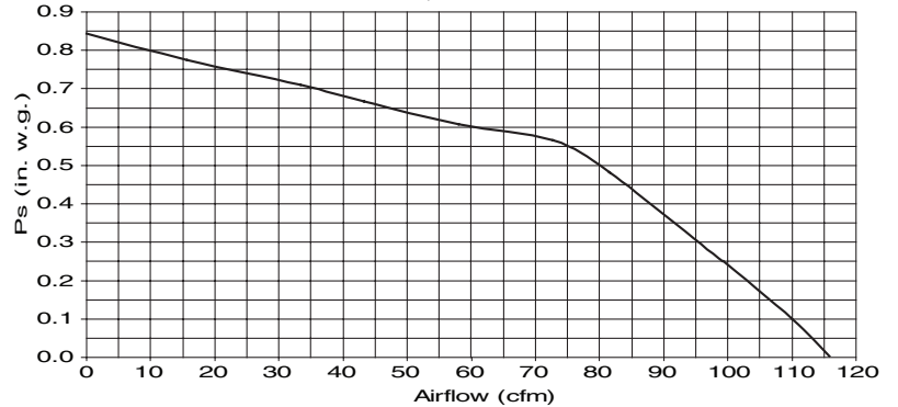
MODEL QTRE110FLT
