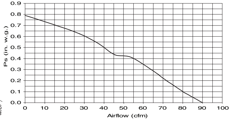
MODEL QTRE080FLT
