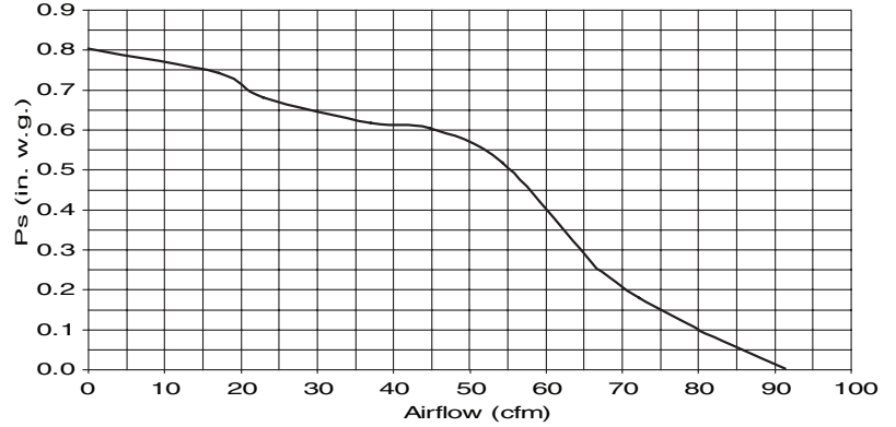
MODEL QTR080L
