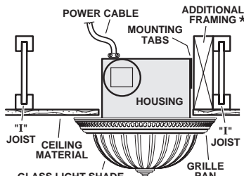
HOUSING MOUNTED TO "1" JOIST Requires additional framing for mounting tabs. Discharge parallel to joists.
