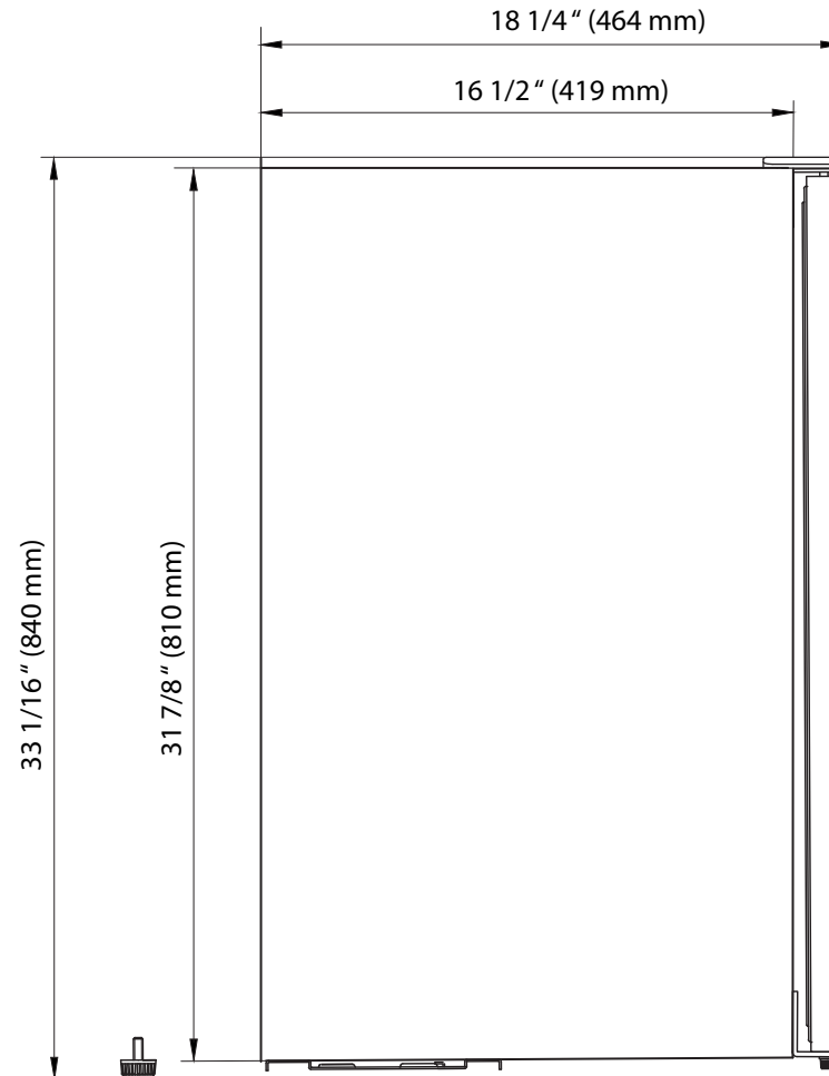
Side View
