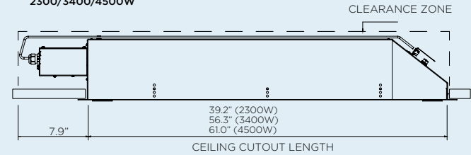
LOW CLEARANCE RECESS KIT 2300/3400/4500W
