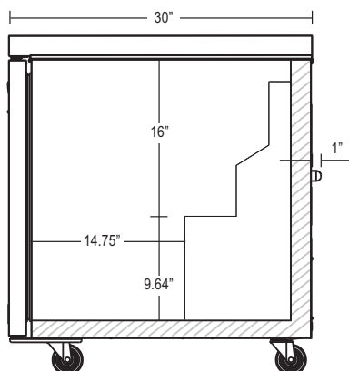
CRMR27-LP SIDE VIEW (Cross Section)
