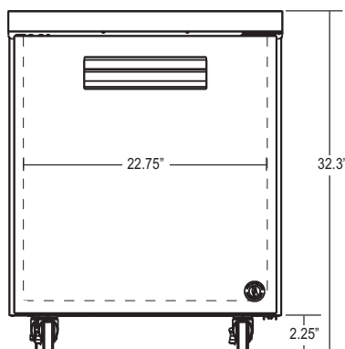
CRMR27-LP FRONT VIEW
