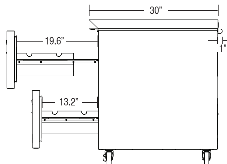
CRMR72-D6 SIDE VIEW
