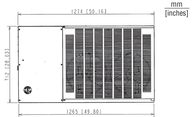
SRK-12H(3) REMOTE CONDENSER
