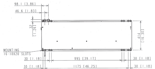
SRK-12H(3) REMOTE CONDENSER
