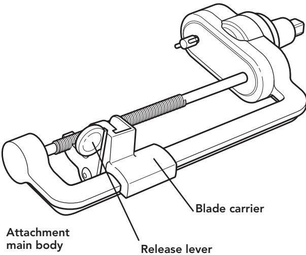
Release lever
