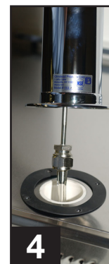
Thread beer line connector to draft arm and secure draft arm to cabinet with rubber gasket under the draft arm.
