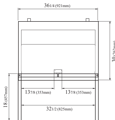
PLAN VIEW
