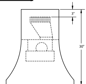
Transition Installed (Side View)
