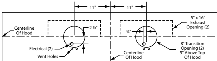
1100 CFM T2+ 200 Dual Blowers (Top View)
