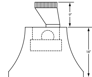
Transition Installed (Side View)
