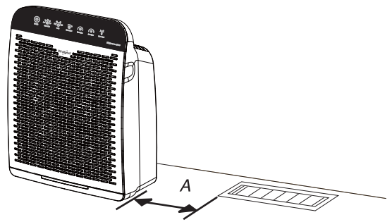
A. 6" (15.2 cm) minimum clearance
