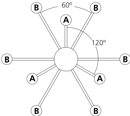
Drawing 2 - Fixture Assembly
