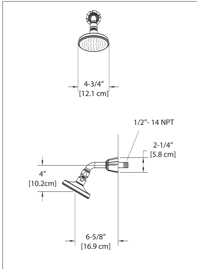
TS970AC - Guinevere™ Showerhead
