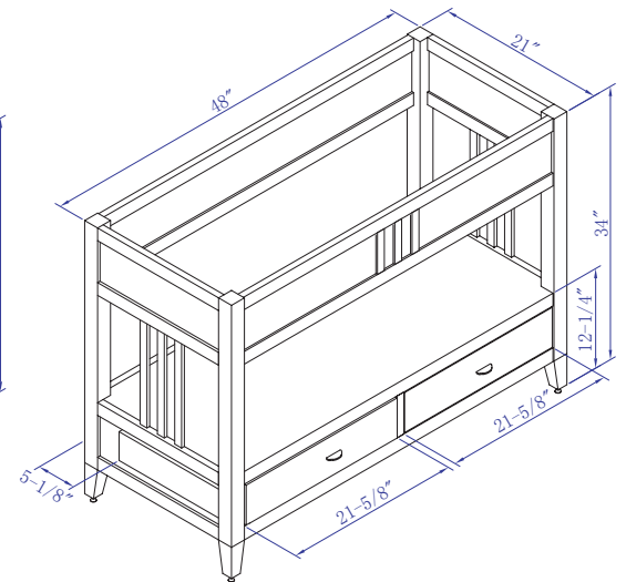
ME4821D Vanity MW4821D Vanity
