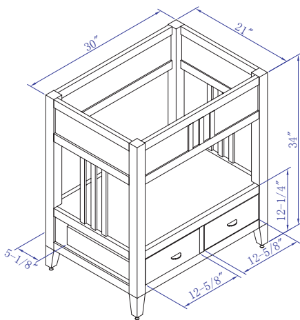
ME3021D Vanity MW3021D Vanity
