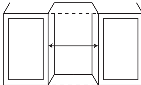
Cutout Width: 15 3/16"
