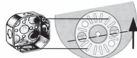
ADAPTOR MOUNTING PLATE SHOWN ROTATED APPROXIMATELY 10^\circ COUNTERCLOCKWISE TO MATCH OUTLET BOX
