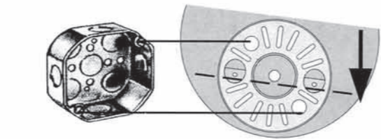
ADAPTOR MOUNTING PLATE SHOWN ROTATED APPROXIMATELY 5^\circ CLOCKWISE TO MATCH OUTLET BOX
