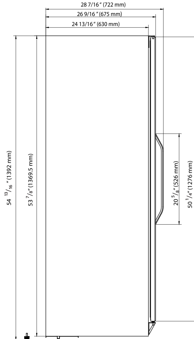
Side View
