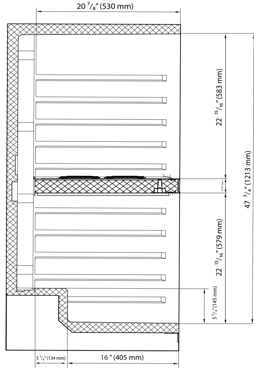
Side View
